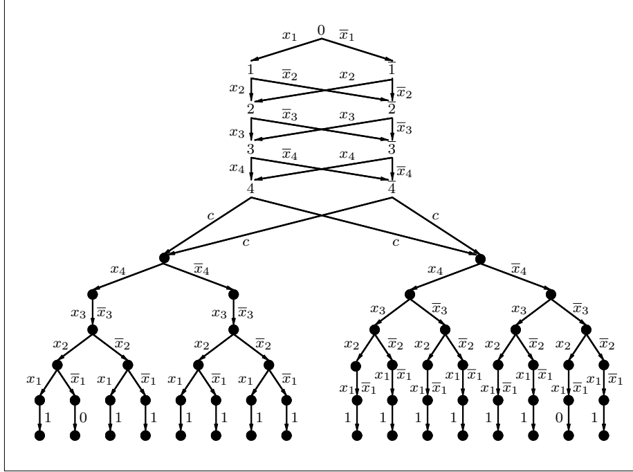
Fig. 3. The transition system for \Phi .
